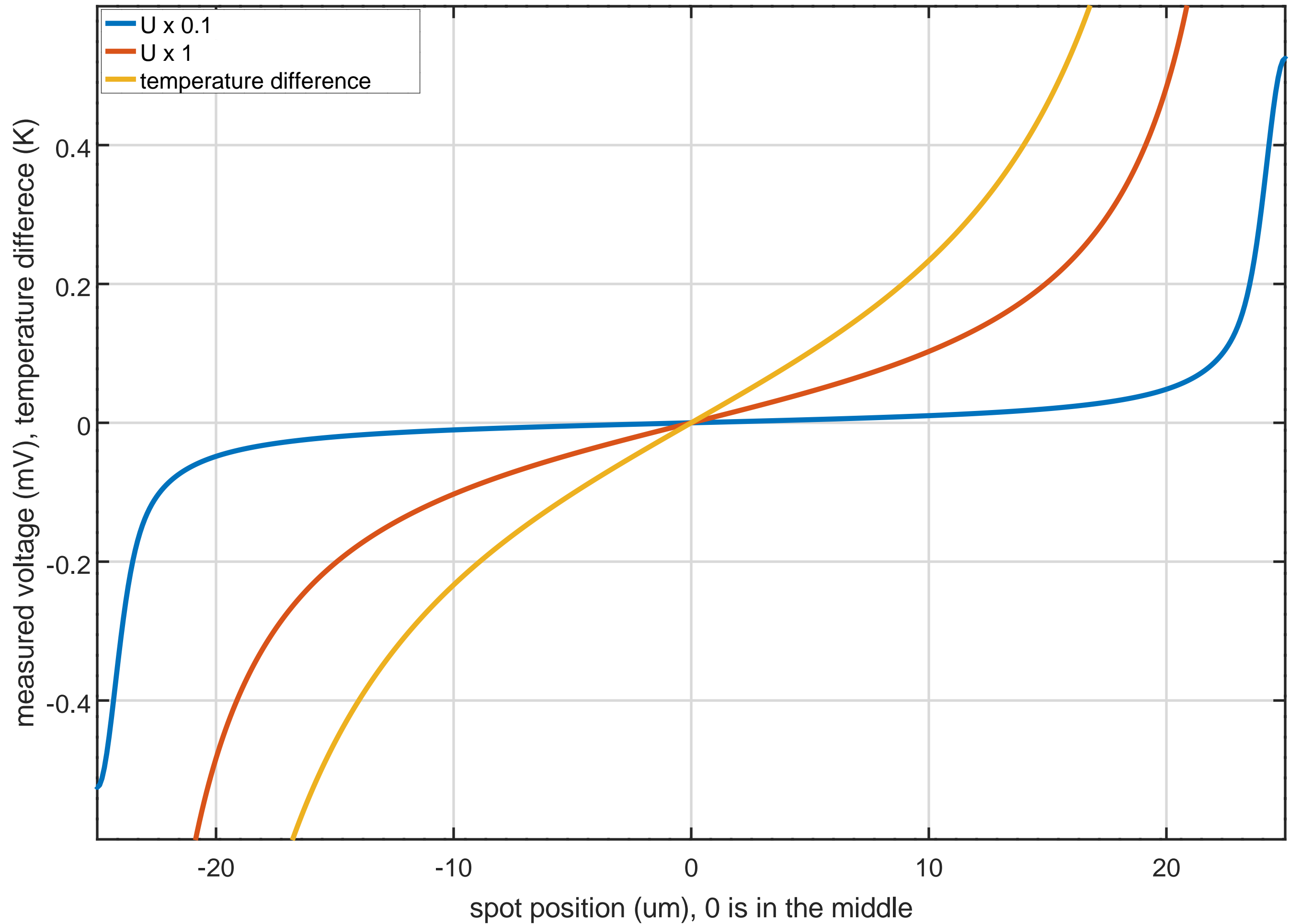
CW absorbed power 6mW, laser spot 1.5um, silicon 0.5mm, 50um between contacts
